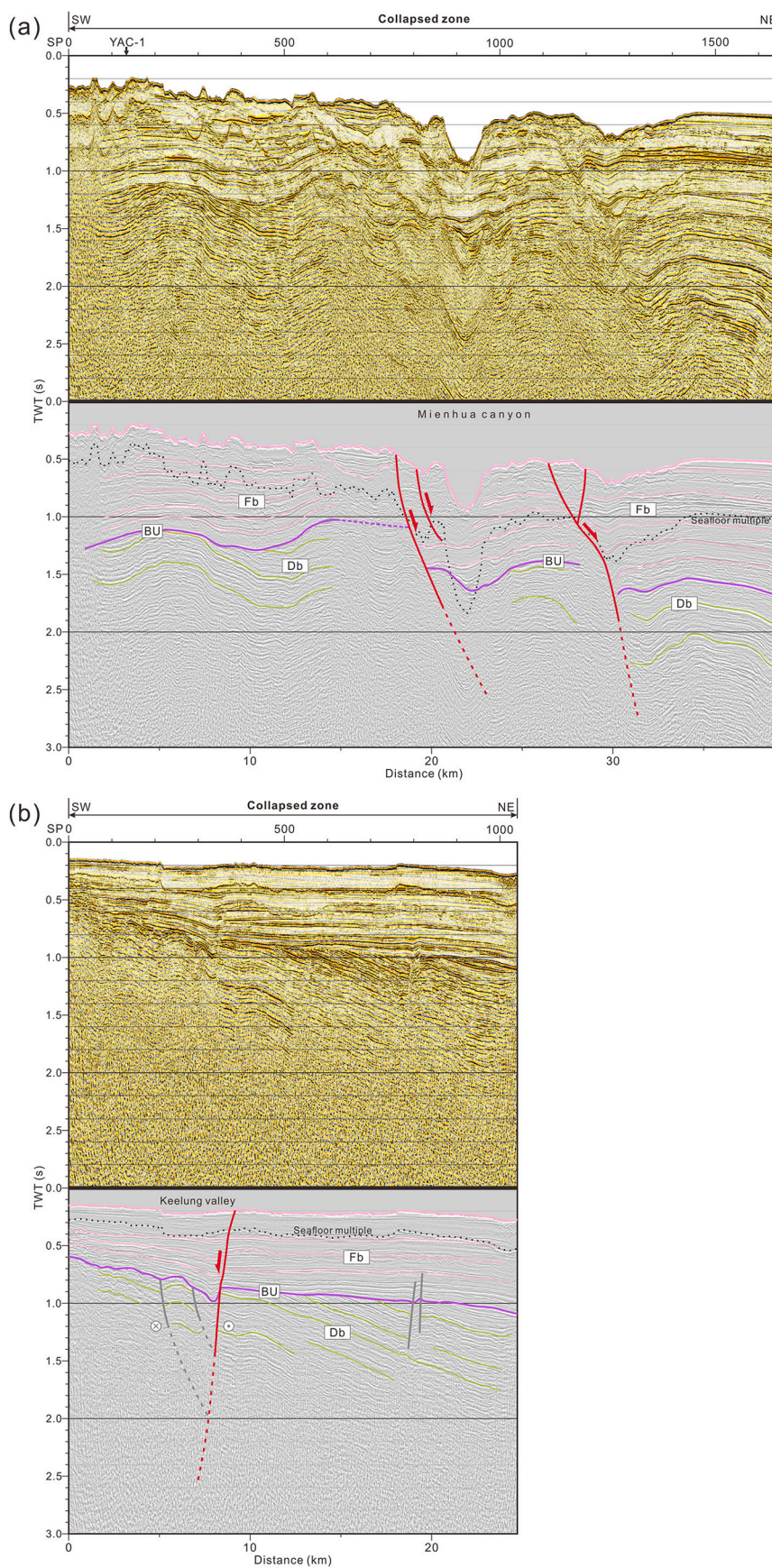
Fig. 6. NE-SW-oriented multi-channel seismic profiles MCS-1048-b06 (a) and MCS-1048-b05 (b) and their interpretations. These two profiles run along the eastern side of the Offshore Shanjiiao Fault. SP: Shot point, TWT: Two-way travel time, OSF: Offshore Shanjiiao Fault. Refer to Fig. 3 for symbols of seismic units and Fig. 2 for locations.
