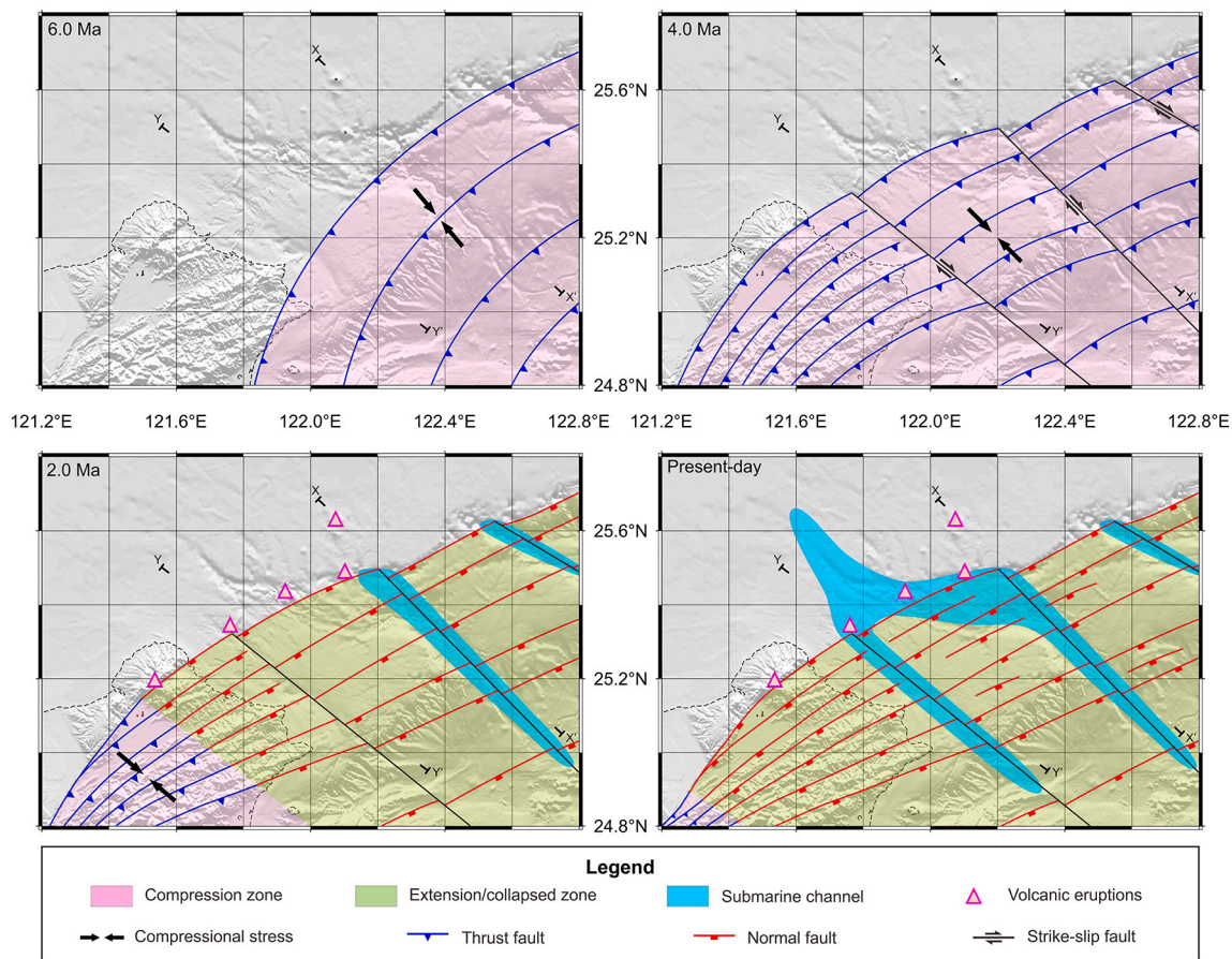
Fig. 9. Cartoons showing the geodynamic evolution in the offshore area of northern Taiwan. The Eurasia plate is fixed. Before ~6 Ma, offshore northern Taiwan was a rifted Eurasian continental margin. At ~6.0 Ma, the uplift of northern offshore Taiwan was due to the collision of the northern Luzon arc of the Philippine Sea plate with the continental margin. The northwesternmost thrust fault located roughly near the present-day Offshore Shanjiao Fault. A series of NW-SE-trending thrust faults were formed due to the oblique collision at about 4.0 Ma. When the northern part of the mountain belt became an extensional setting, the NE-SW-trending thrust faults were reactivated as normal faults. Subsequently, the magma may have extruded along normal fault systems to form submarine volcanoes and volcanic islets since 2.5 Ma. The NW-SE-trending strike-slip faults also facilitated the development of the submarine channels. The Offshore Shanjiao Fault is the westernmost boundary of the crustal extensional regime in response to the opening of the southern Okinawa Trough since 2 Ma. The normal fault system continues its activity in the collapsed zone until the present-day. Cross-sections of XX' and YY' are shown in Fig. 10.
